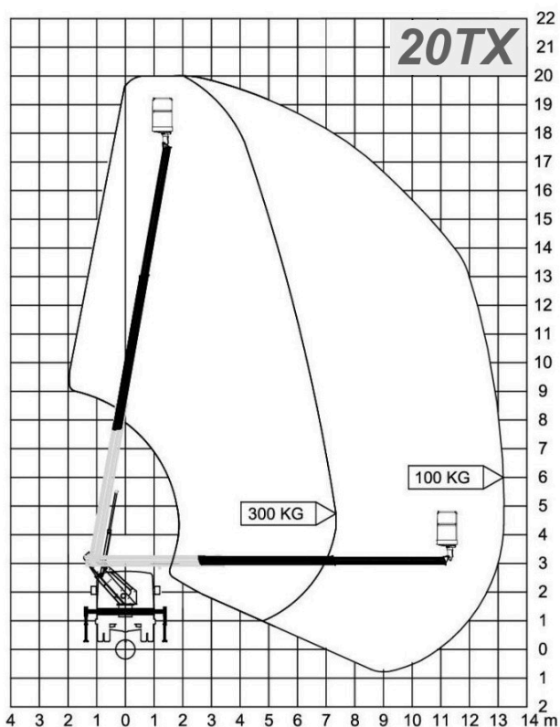
Cela Essential 20TX — delovni diagram
