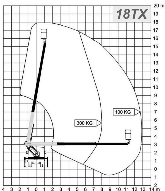
Cela Essential 18TX — working diagram
